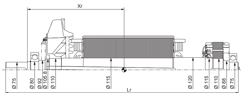
Centre of gravity: X_r (mm), Rotor length: L_r (mm), Weight: M (kg), Moment of inertia: J ( \text{kgm}^2 ): ( 4J = MD^2 )
